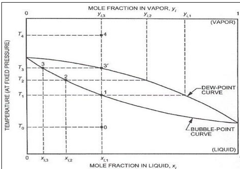
Fig 7: Temperature –concentration (T-x) diagram zeotropic mixture
