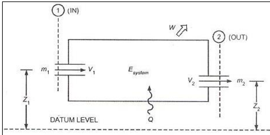
Fig 6: Energy flows in general thermodynamic system
