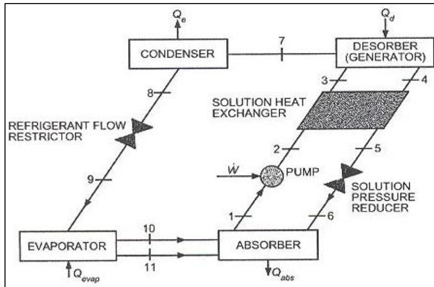
Fig 13: Single-effect absorption cycle
