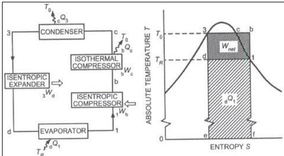
Fig 9: Carnot vapours compression cycle
