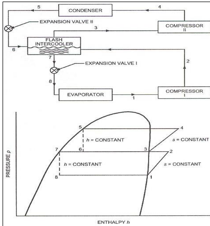
Fig 11: Schematic and pressure-enthalpy diagram for dual-compression, dual-expansion cycles
