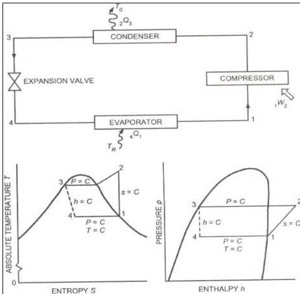
Fig 10: Theoretical single-stage vapours compression refrigeration cycle
