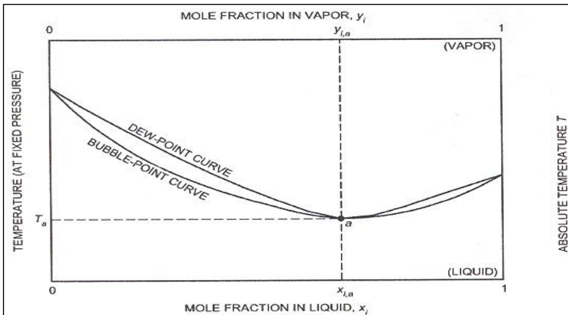
Fig 8: Azeotropic behaviour shown on T-x diagram
