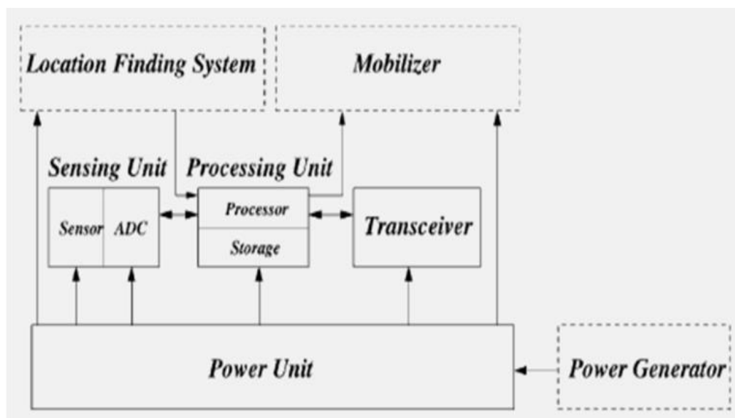
Fig. 2: Components of sensor node
